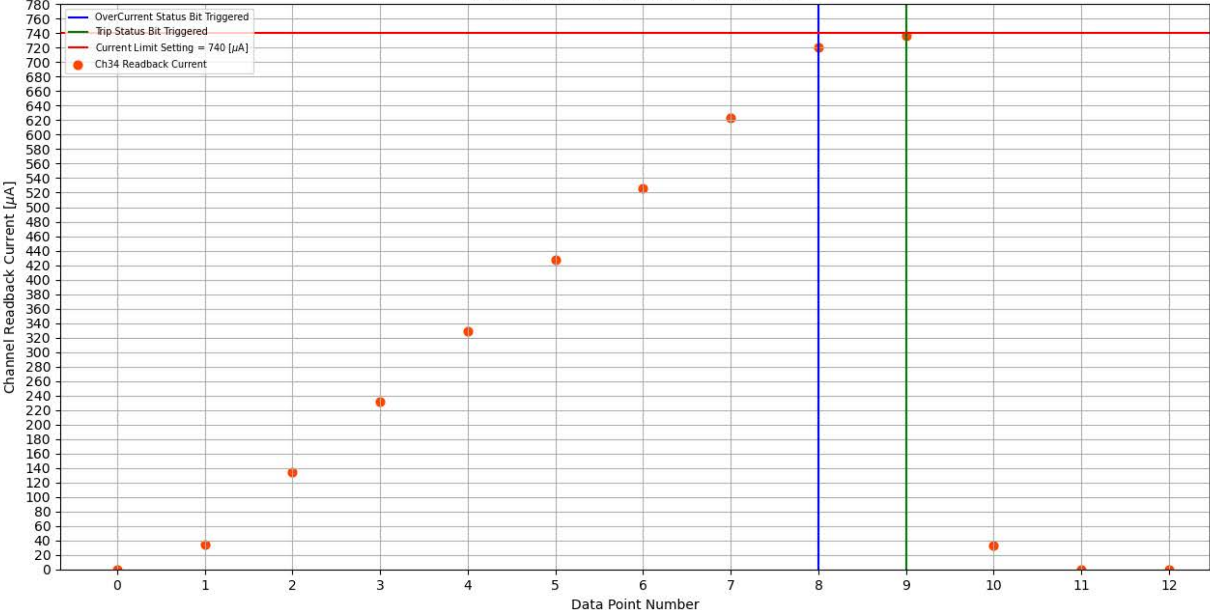
Module 184, Slot 2, Channel 34 Trip Test
