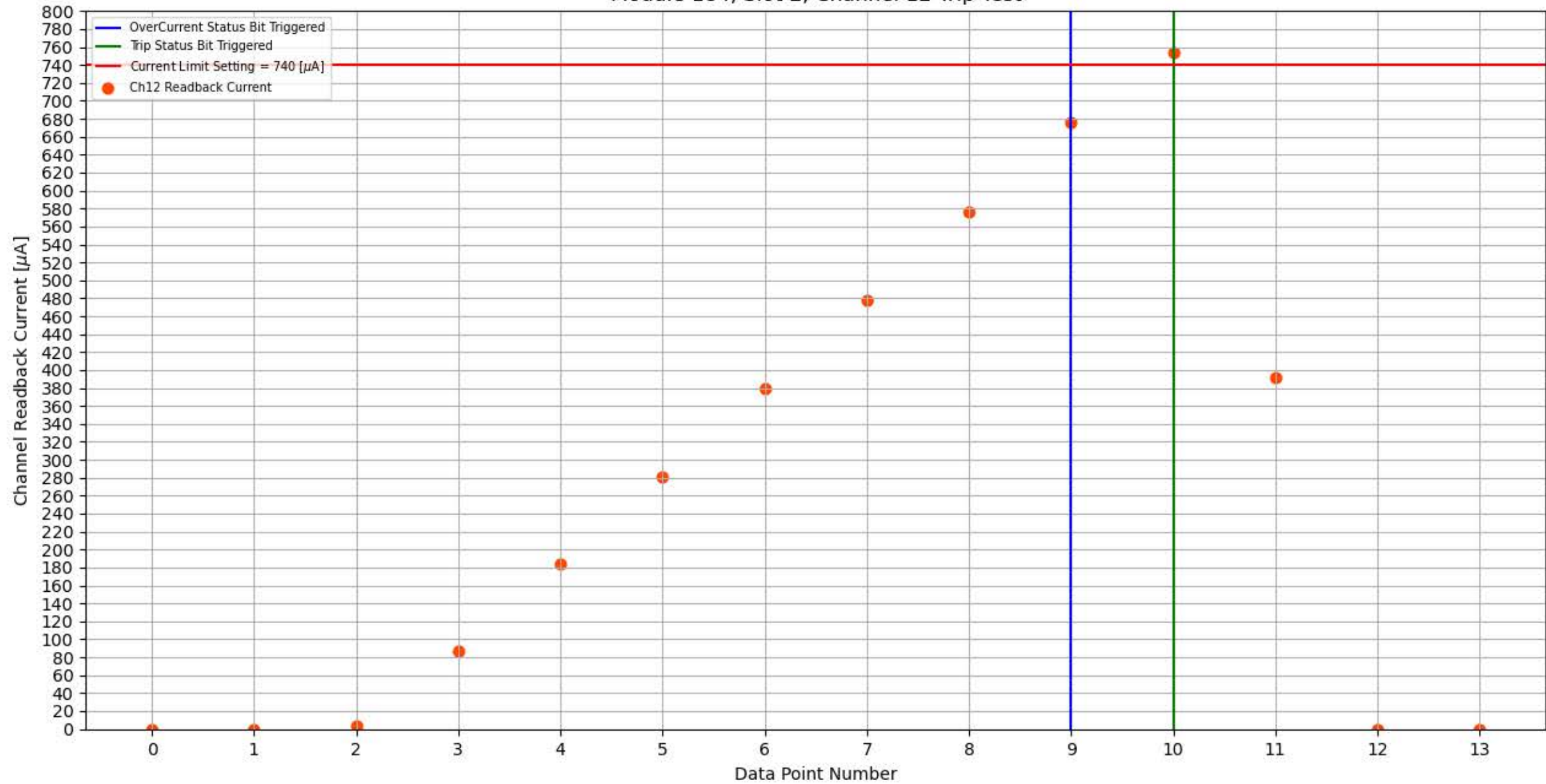
Module 184, Slot 2, Channel 12 Trip Test
