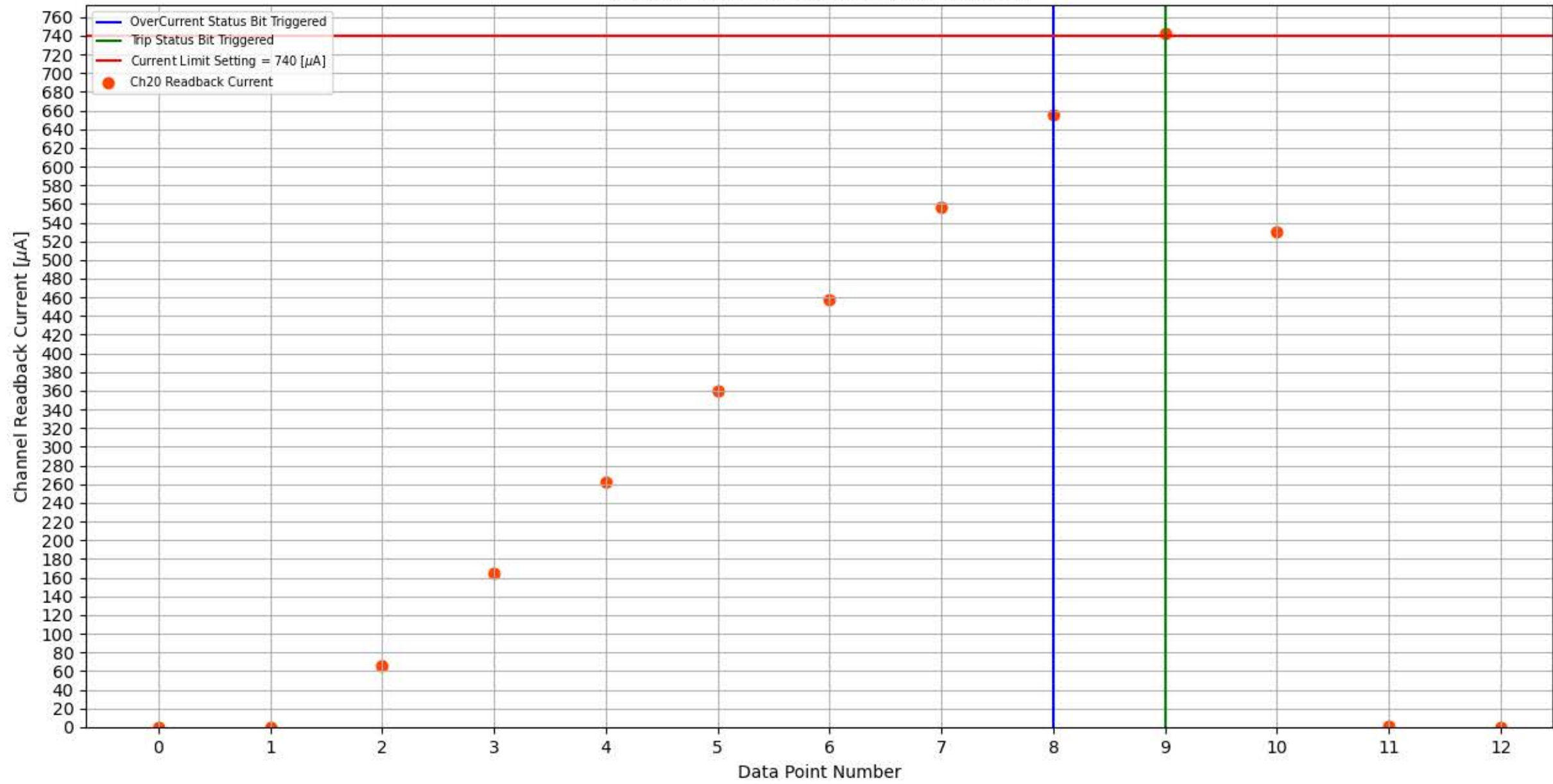
Module 184, Slot 2, Channel 20 Trip Test
