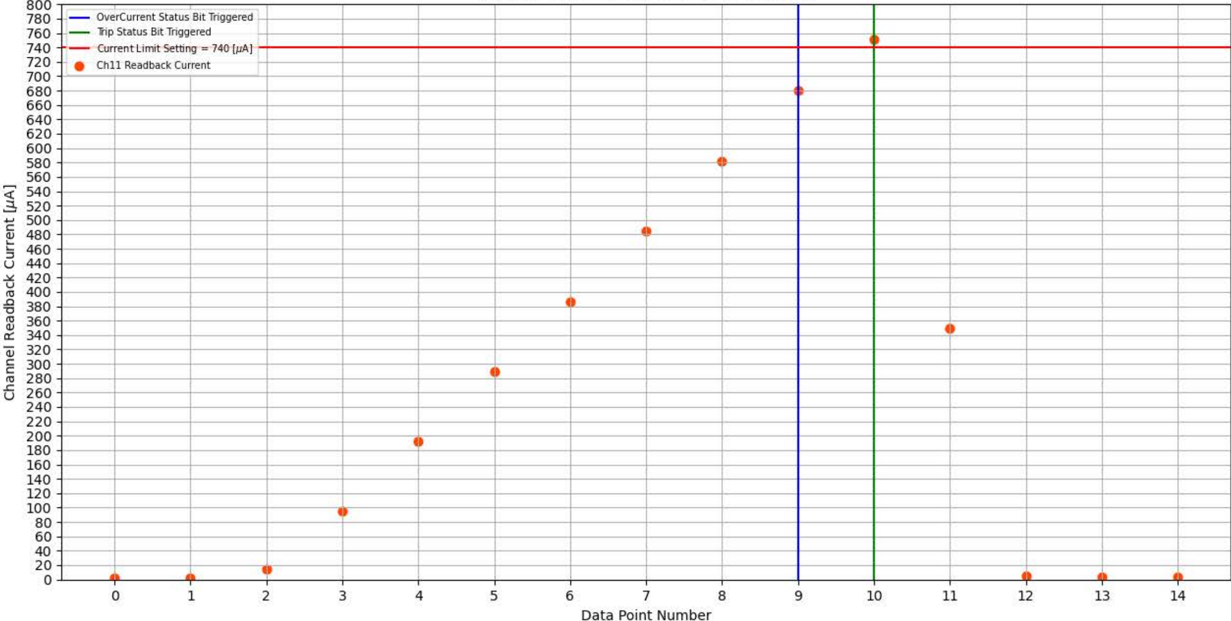
Module 184, Slot 2, Channel 11 Trip Test
