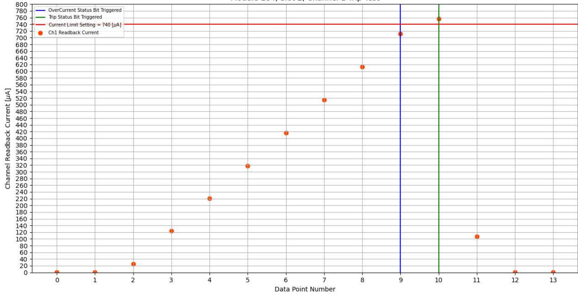
Module 184, Slot 2, Channel 1 Trip Test
