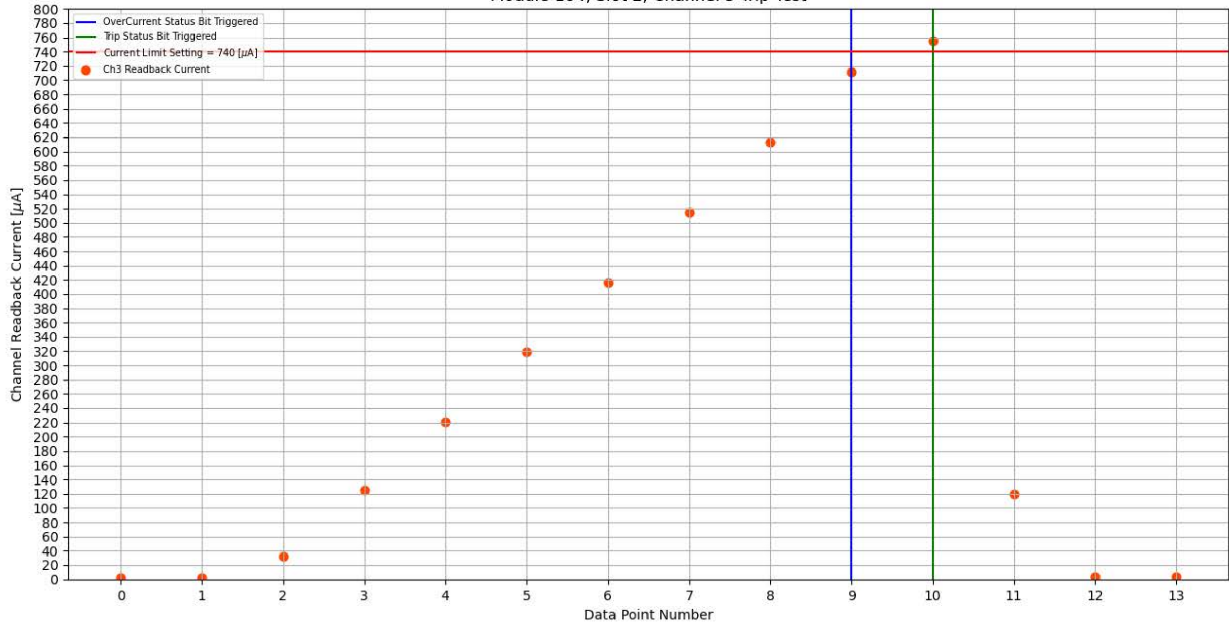
Module 184, Slot 2, Channel 3 Trip Test
