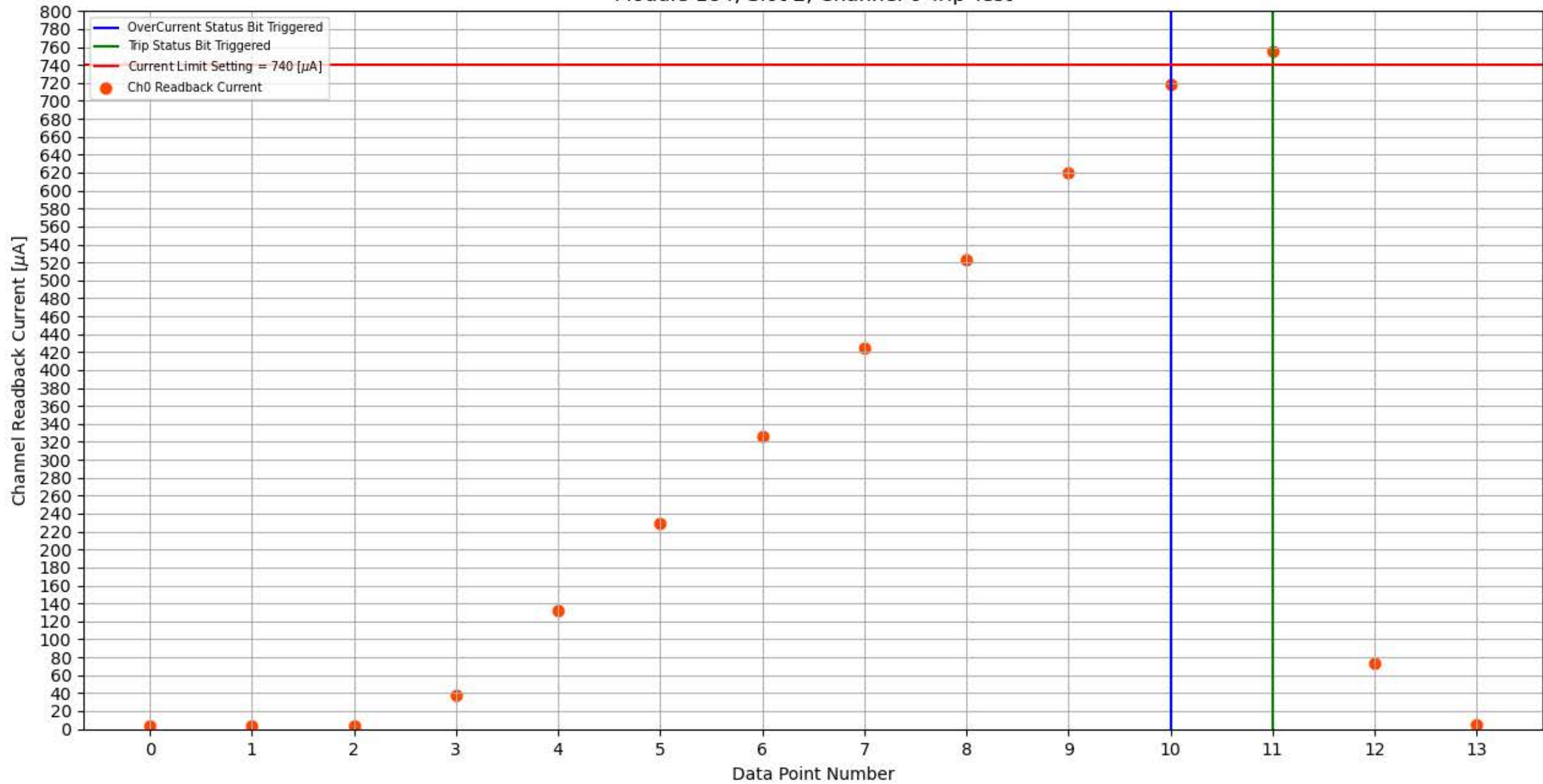
Module 184, Slot 2, Channel 0 Trip Test
