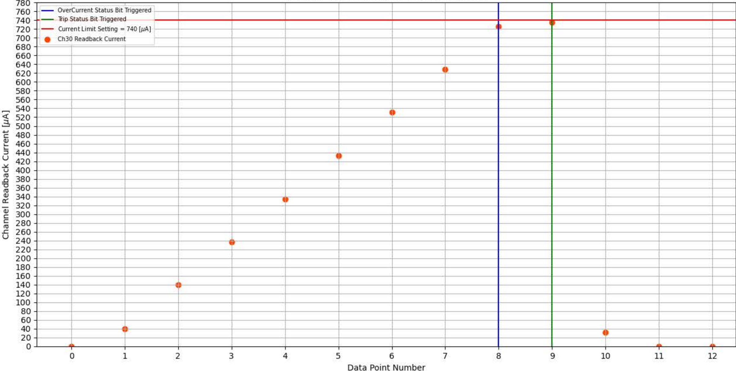
Module 184, Slot 2, Channel 30 Trip Test
