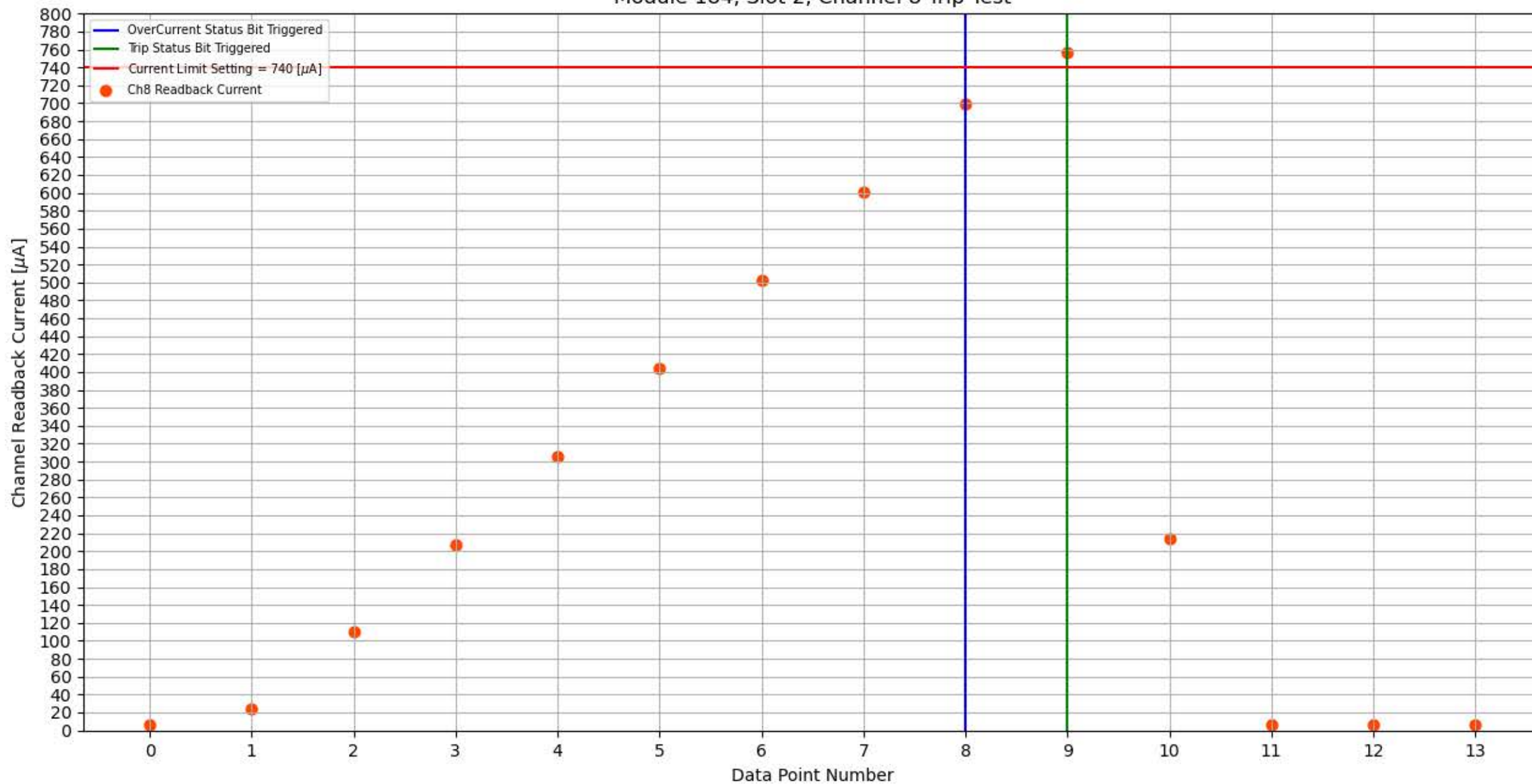
Module 184, Slot 2, Channel 8 Trip Test
