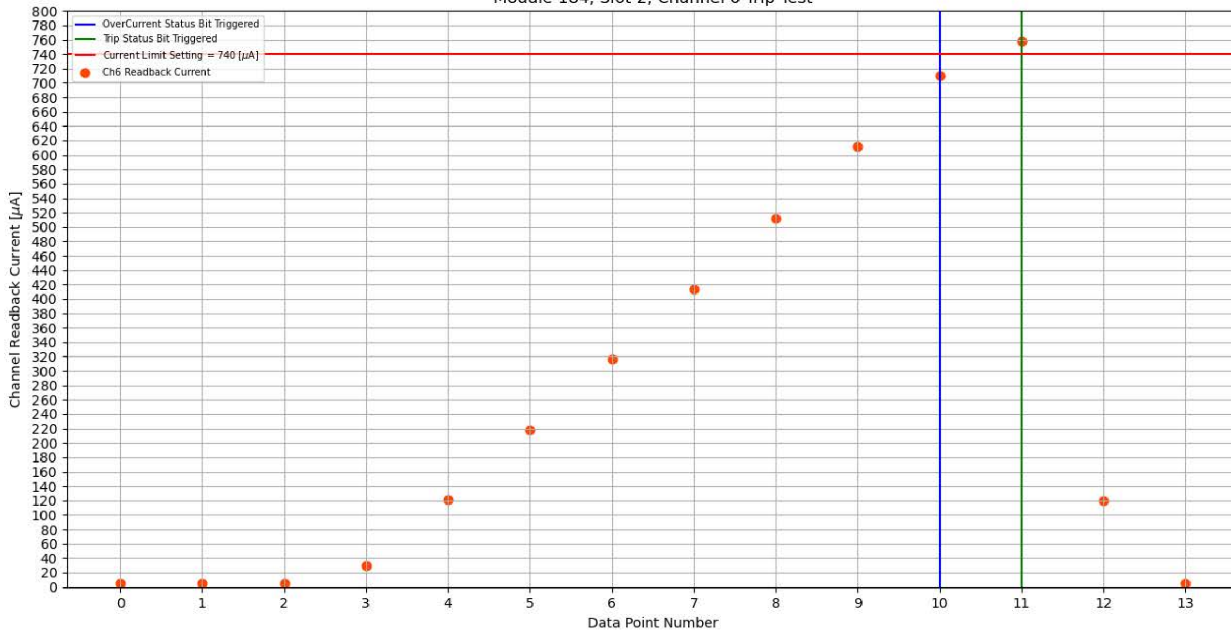
Module 184, Slot 2, Channel 6 Trip Test
