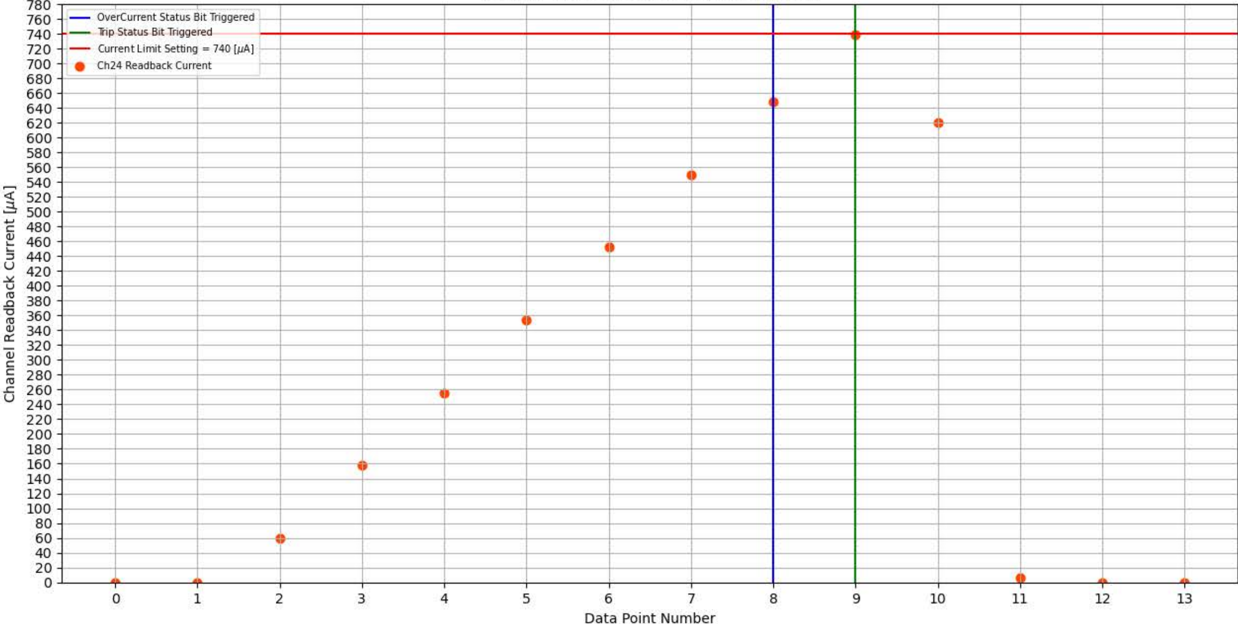
Module 184, Slot 2, Channel 24 Trip Test
