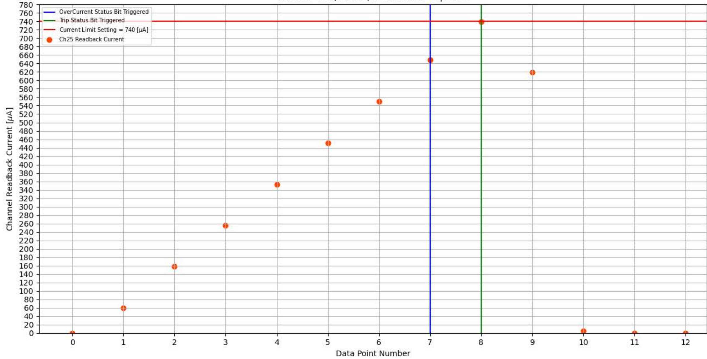
Module 184, Slot 2, Channel 25 Trip Test
