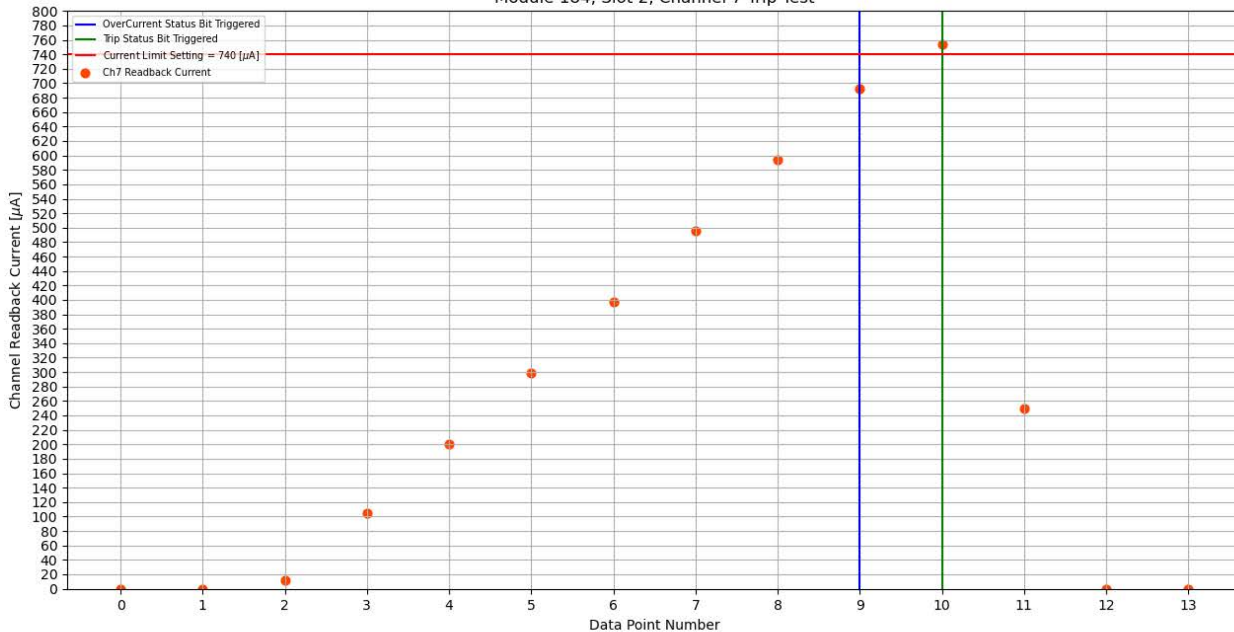
Module 184, Slot 2, Channel 7 Trip Test
