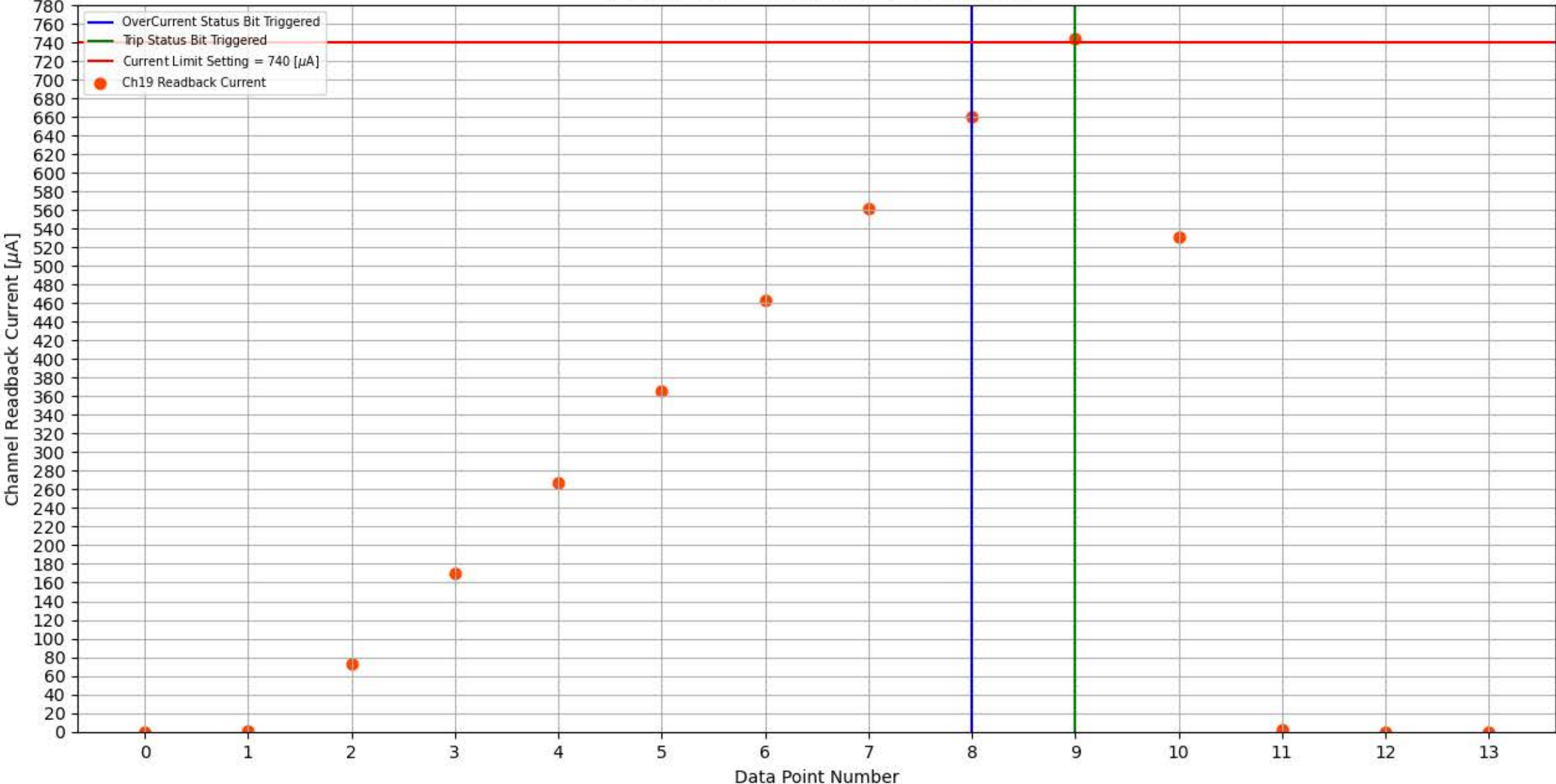
Module 184, Slot 2, Channel 19 Trip Test
