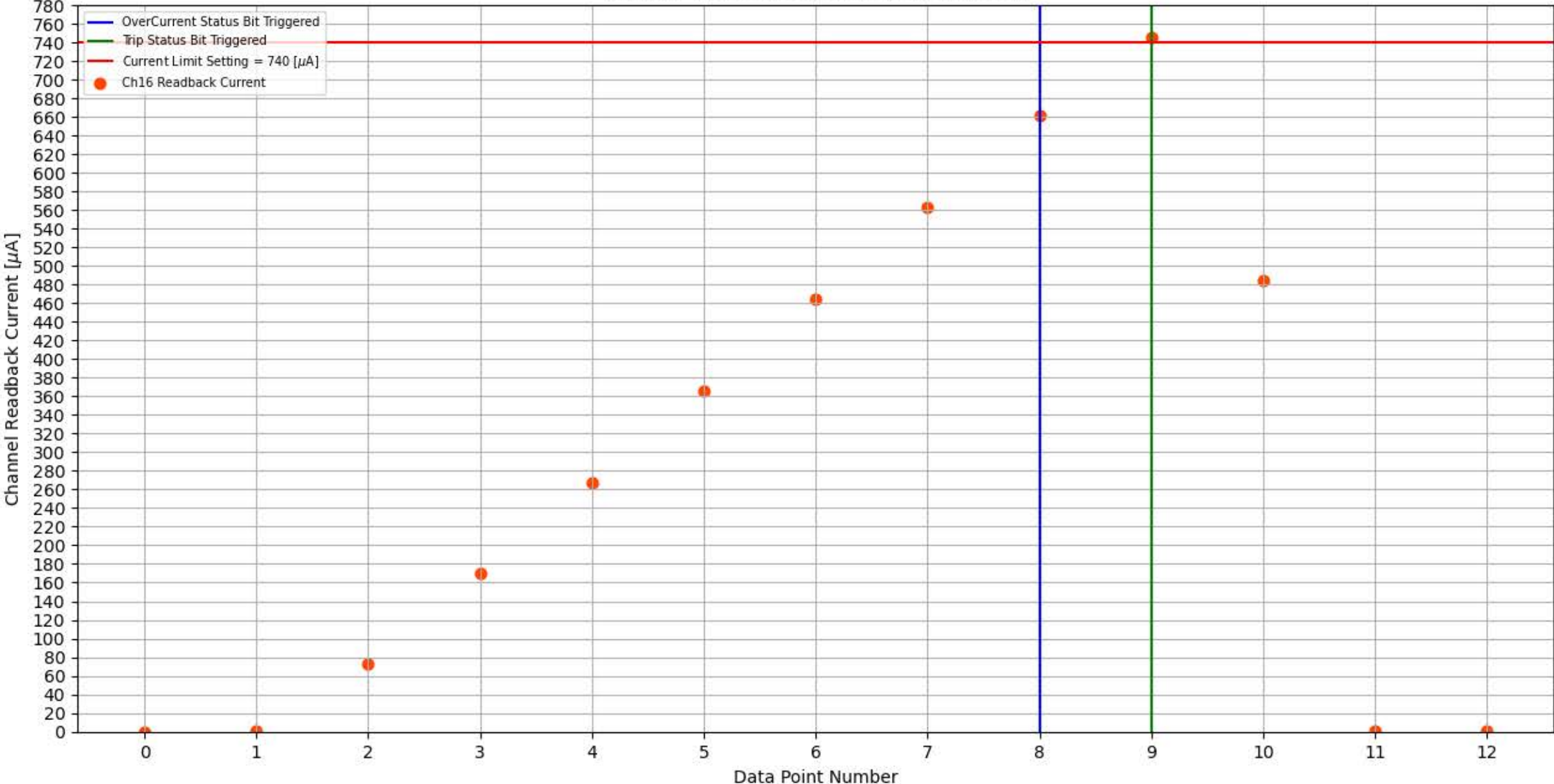
Module 184, Slot 2, Channel 16 Trip Test
