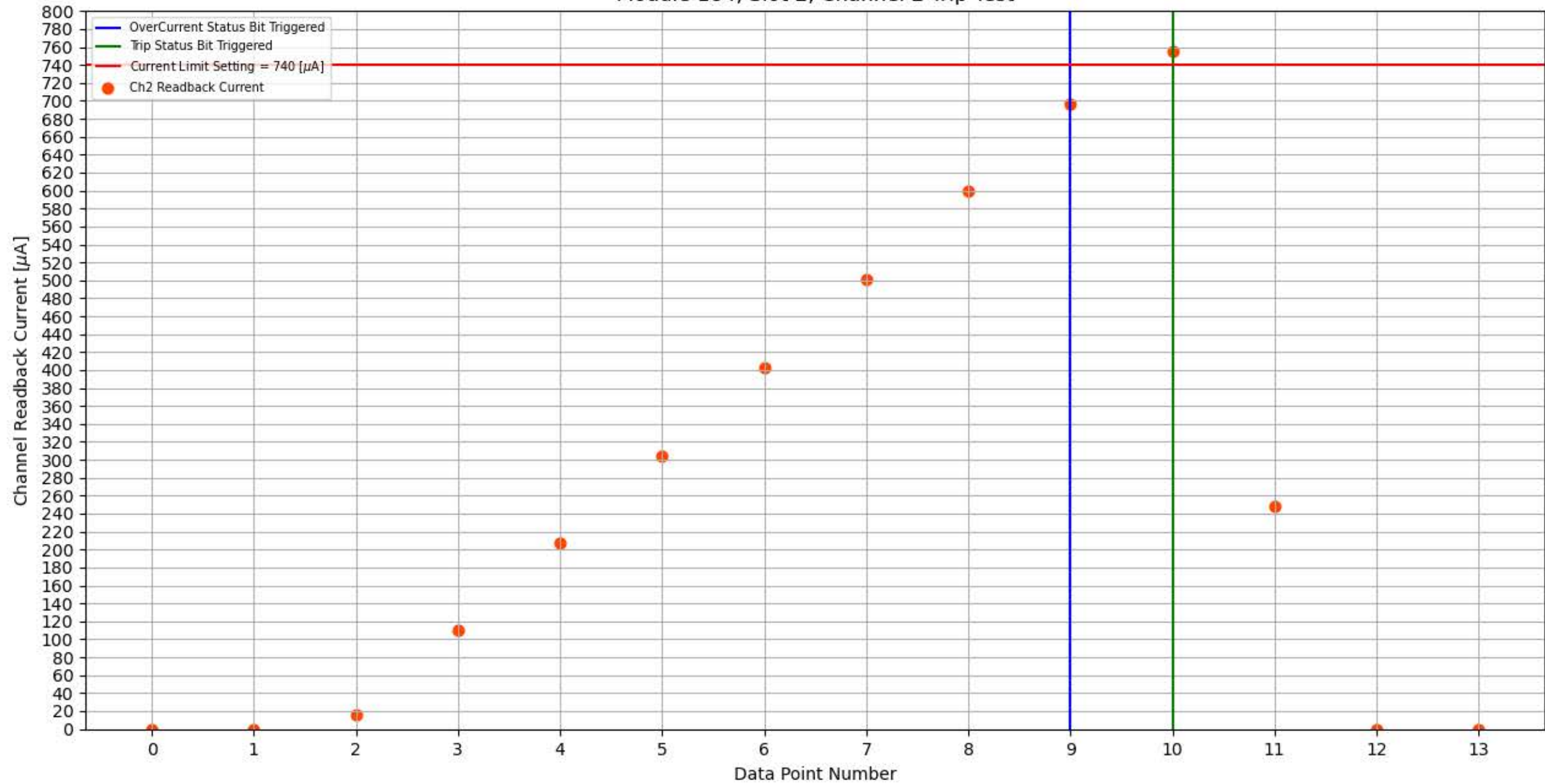
Module 184, Slot 2, Channel 2 Trip Test
