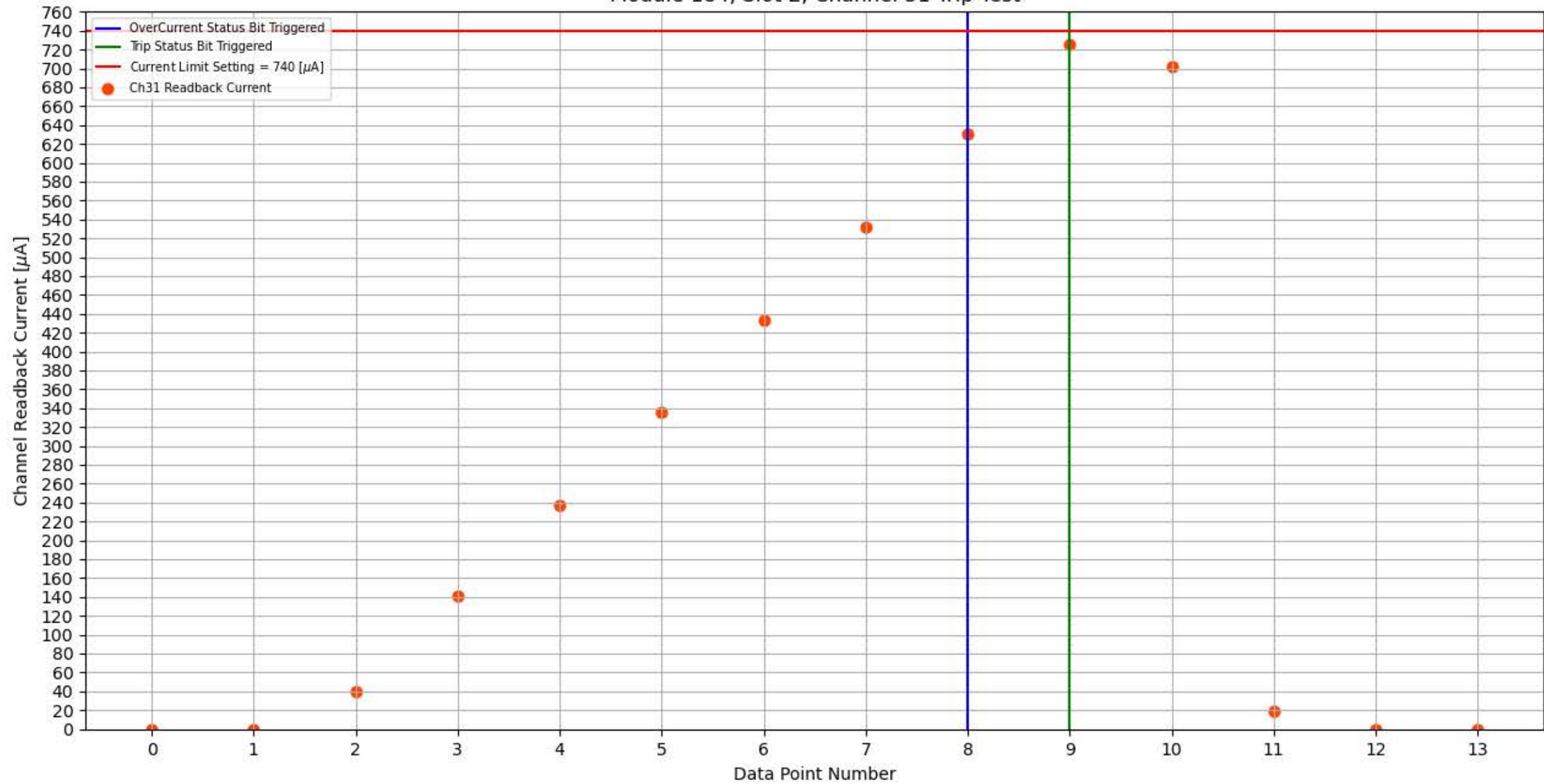
Module 184, Slot 2, Channel 31 Trip Test
