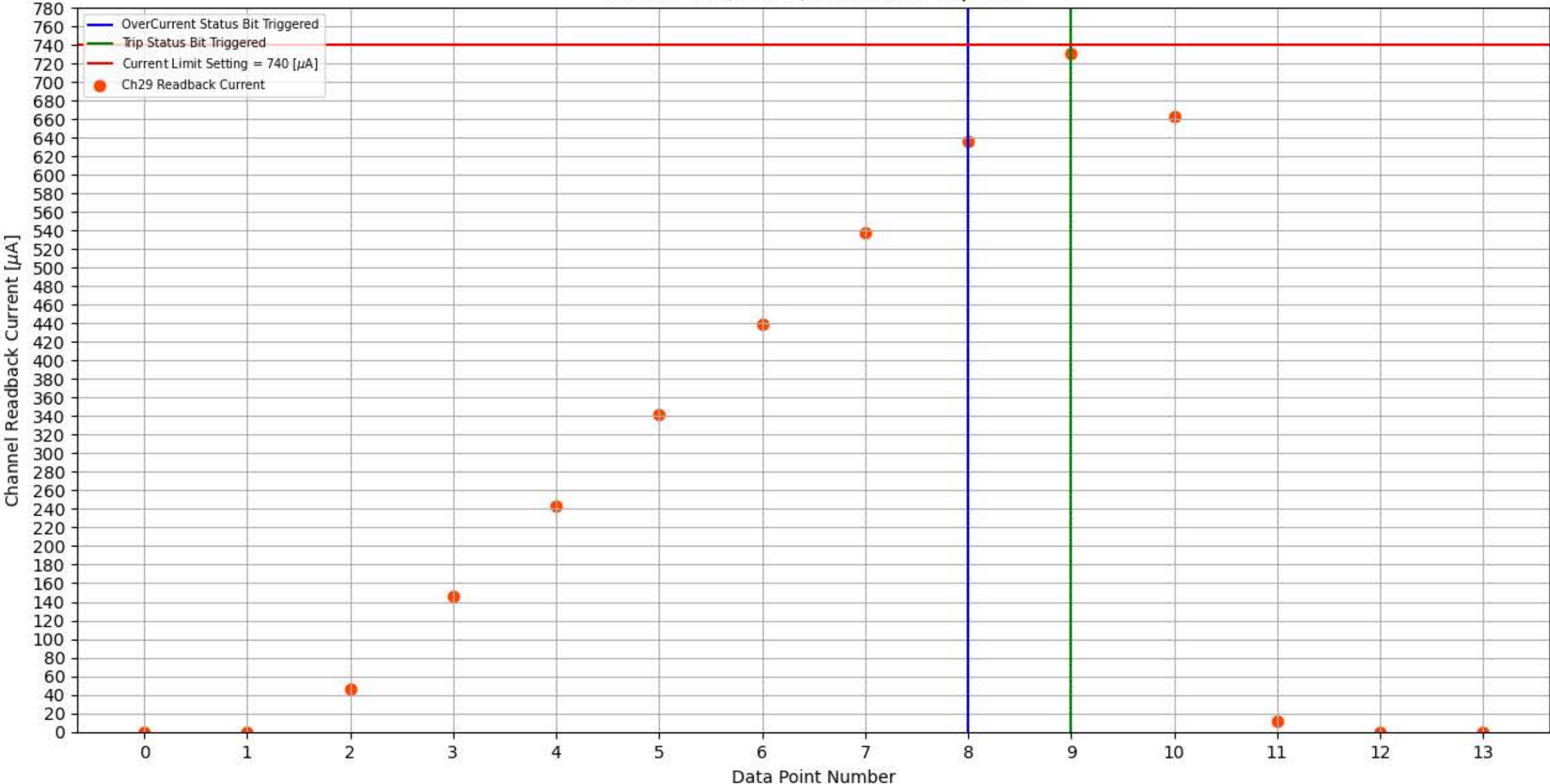
Module 184, Slot 2, Channel 29 Trip Test
