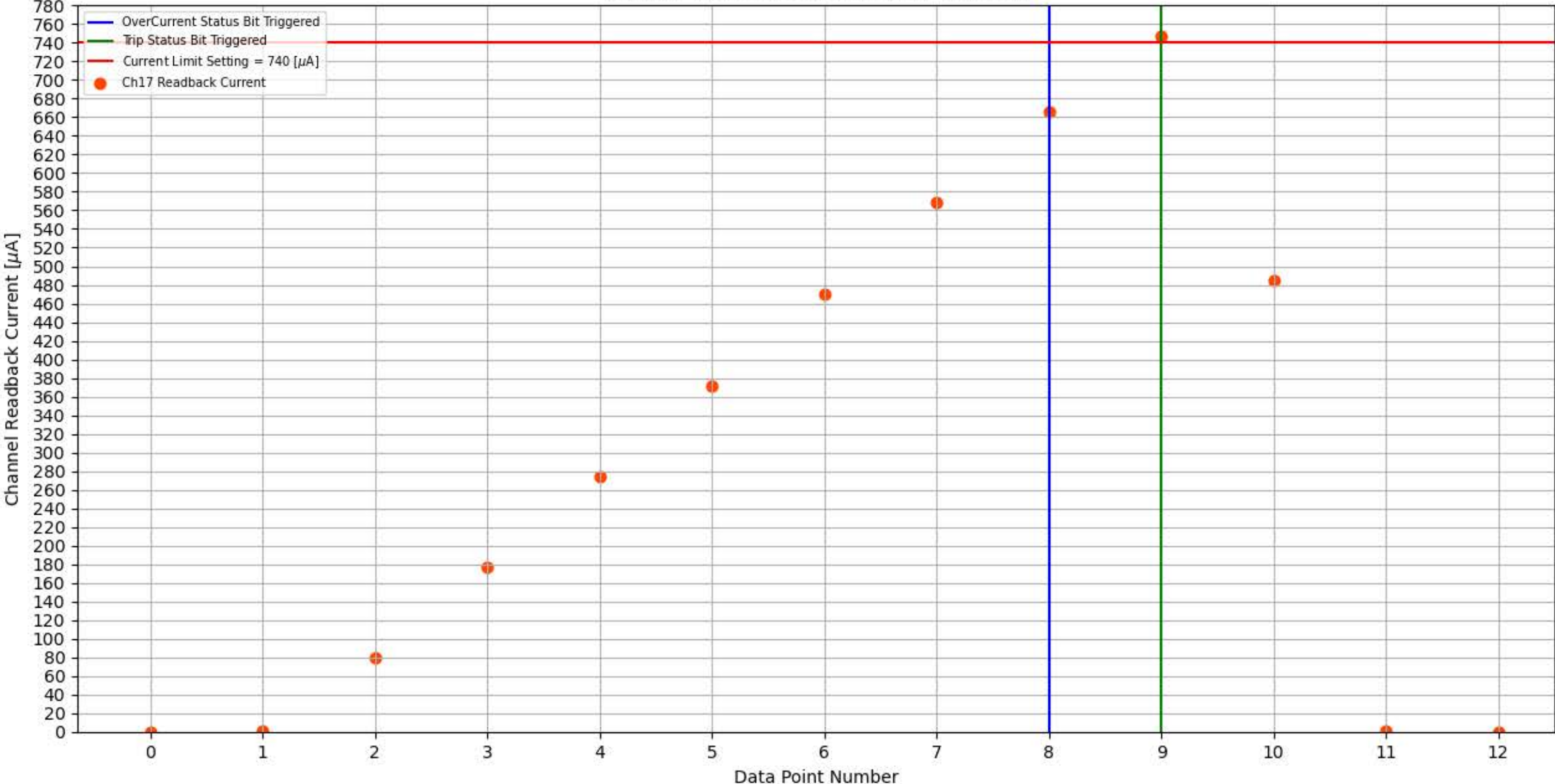
Module 184, Slot 2, Channel 17 Trip Test
