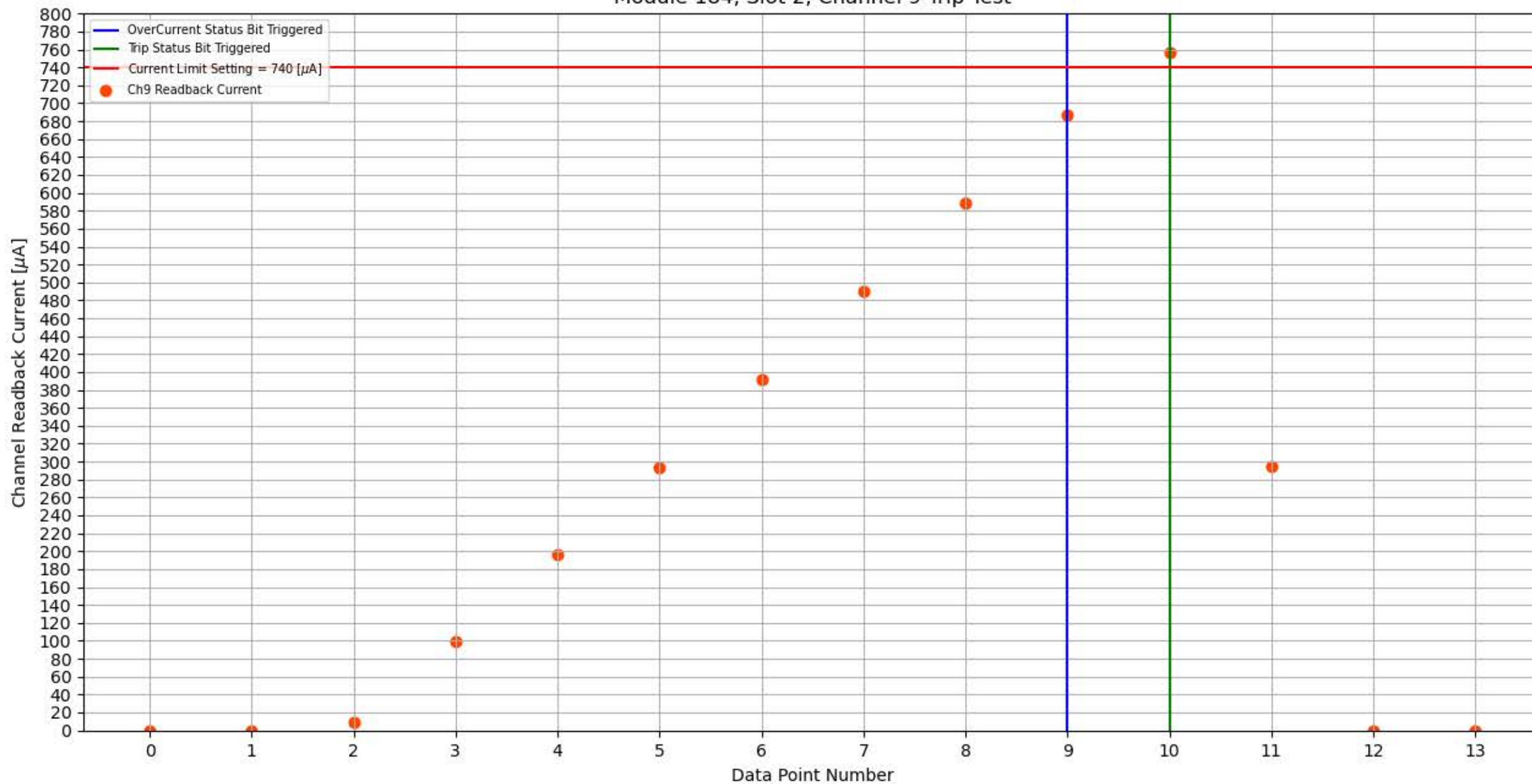
Module 184, Slot 2, Channel 9 Trip Test
