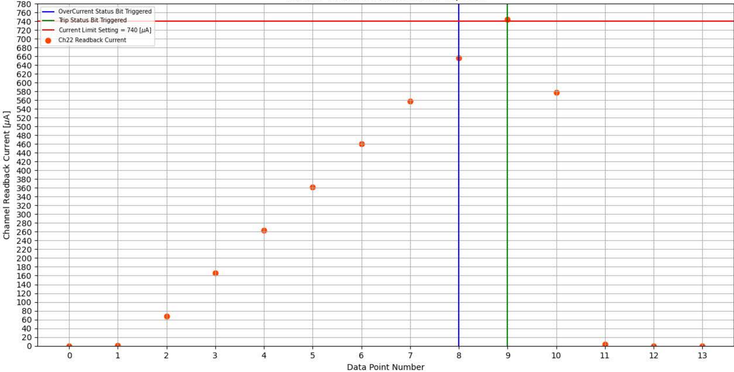
Module 184, Slot 2, Channel 22 Trip Test
