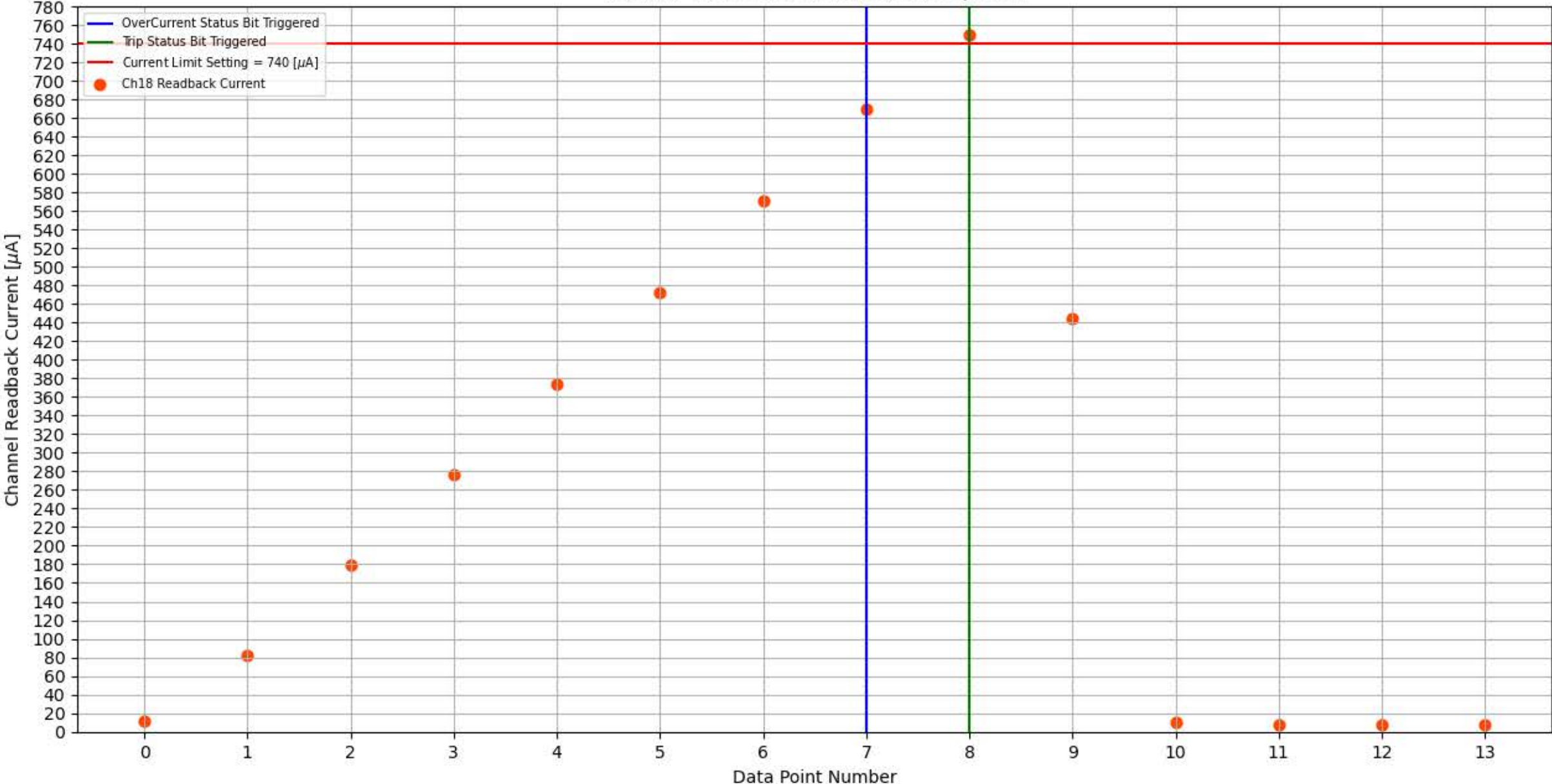
Module 184, Slot 2, Channel 18 Trip Test
