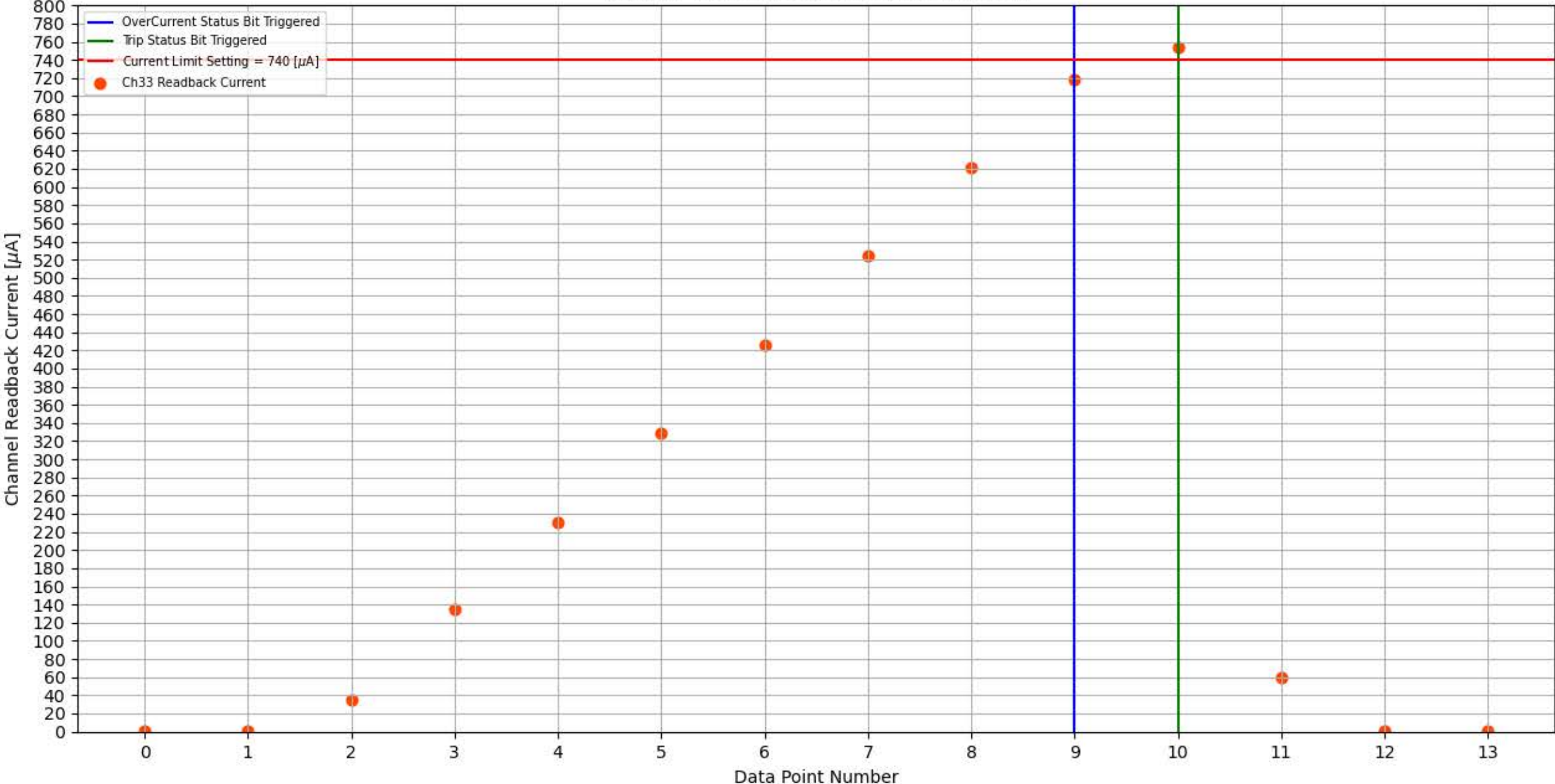
Module 184, Slot 2, Channel 33 Trip Test
