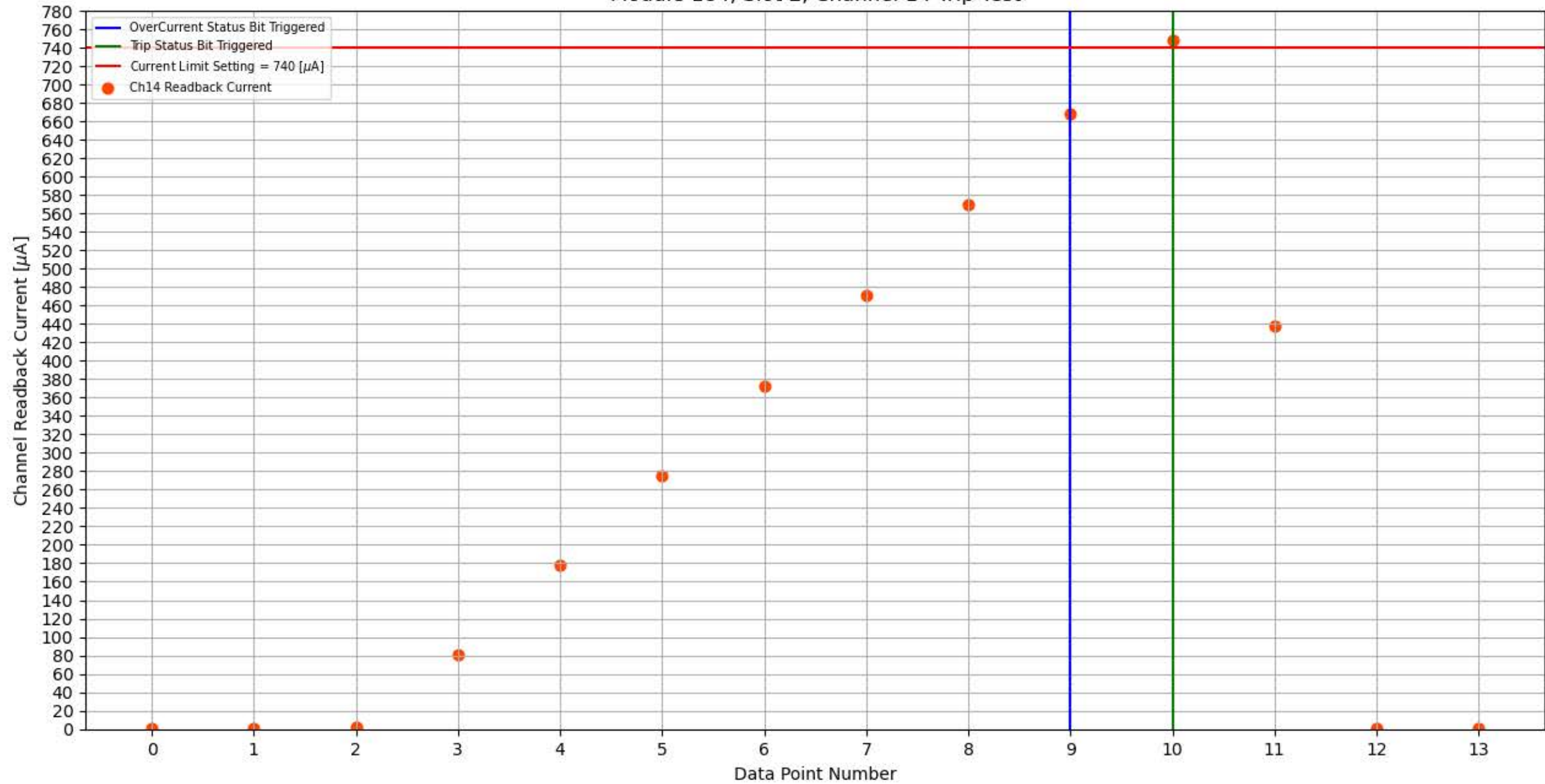
Module 184, Slot 2, Channel 14 Trip Test
