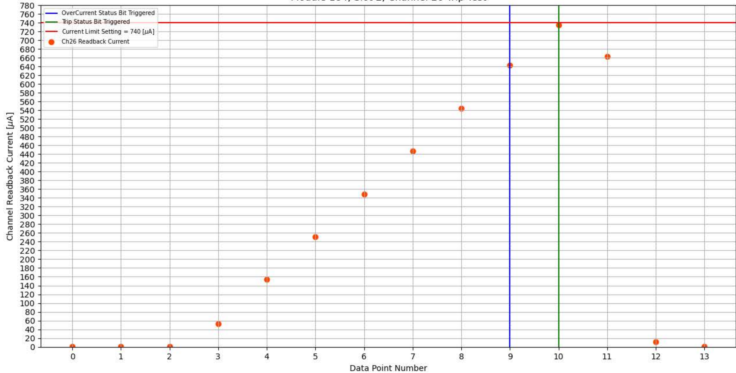
Module 184, Slot 2, Channel 26 Trip Test
