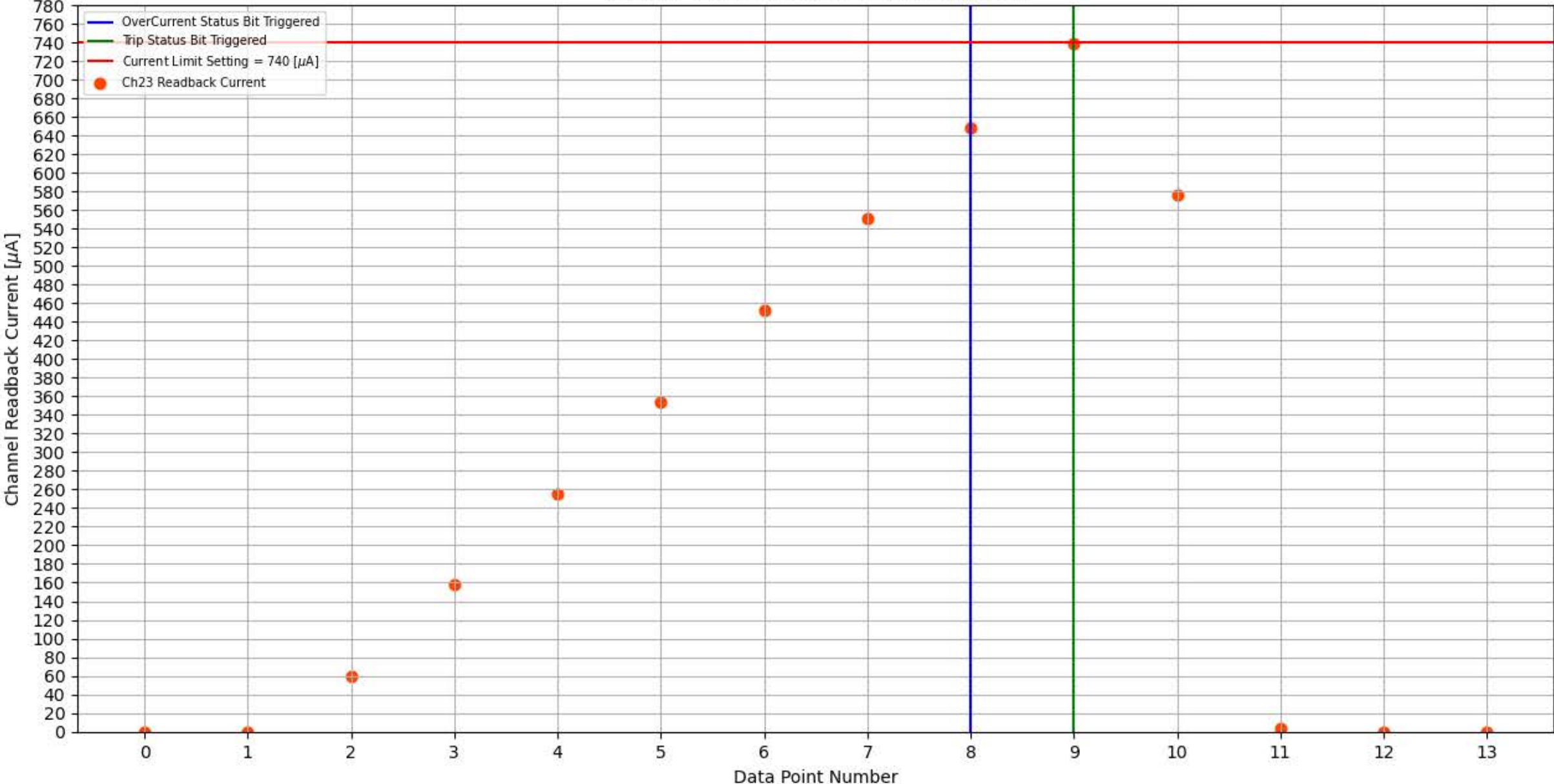
Module 184, Slot 2, Channel 23 Trip Test
