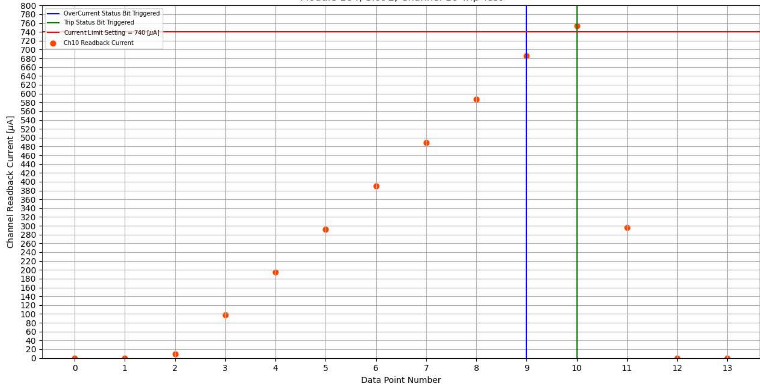
Module 184, Slot 2, Channel 10 Trip Test
