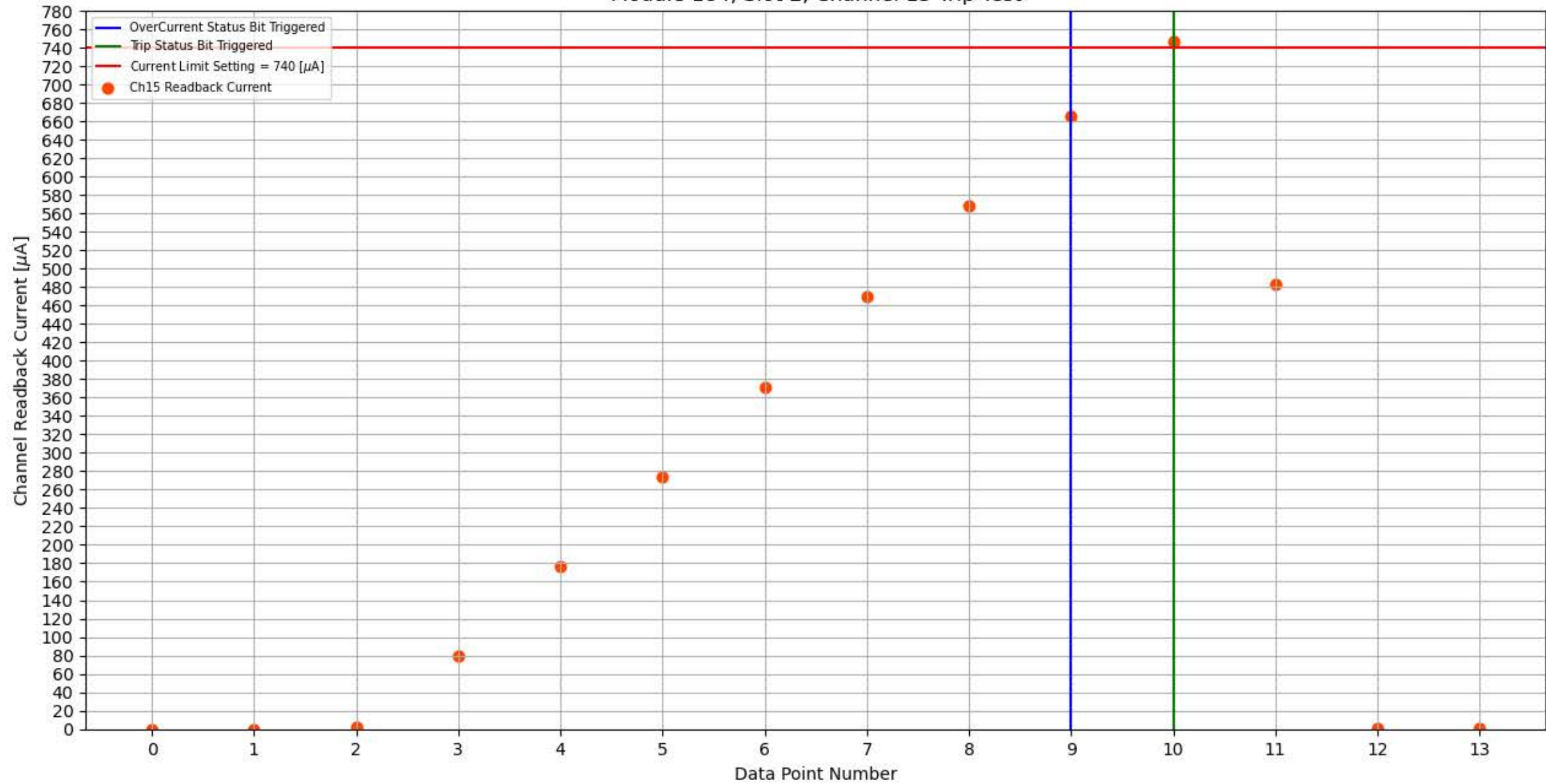
Module 184, Slot 2, Channel 15 Trip Test
