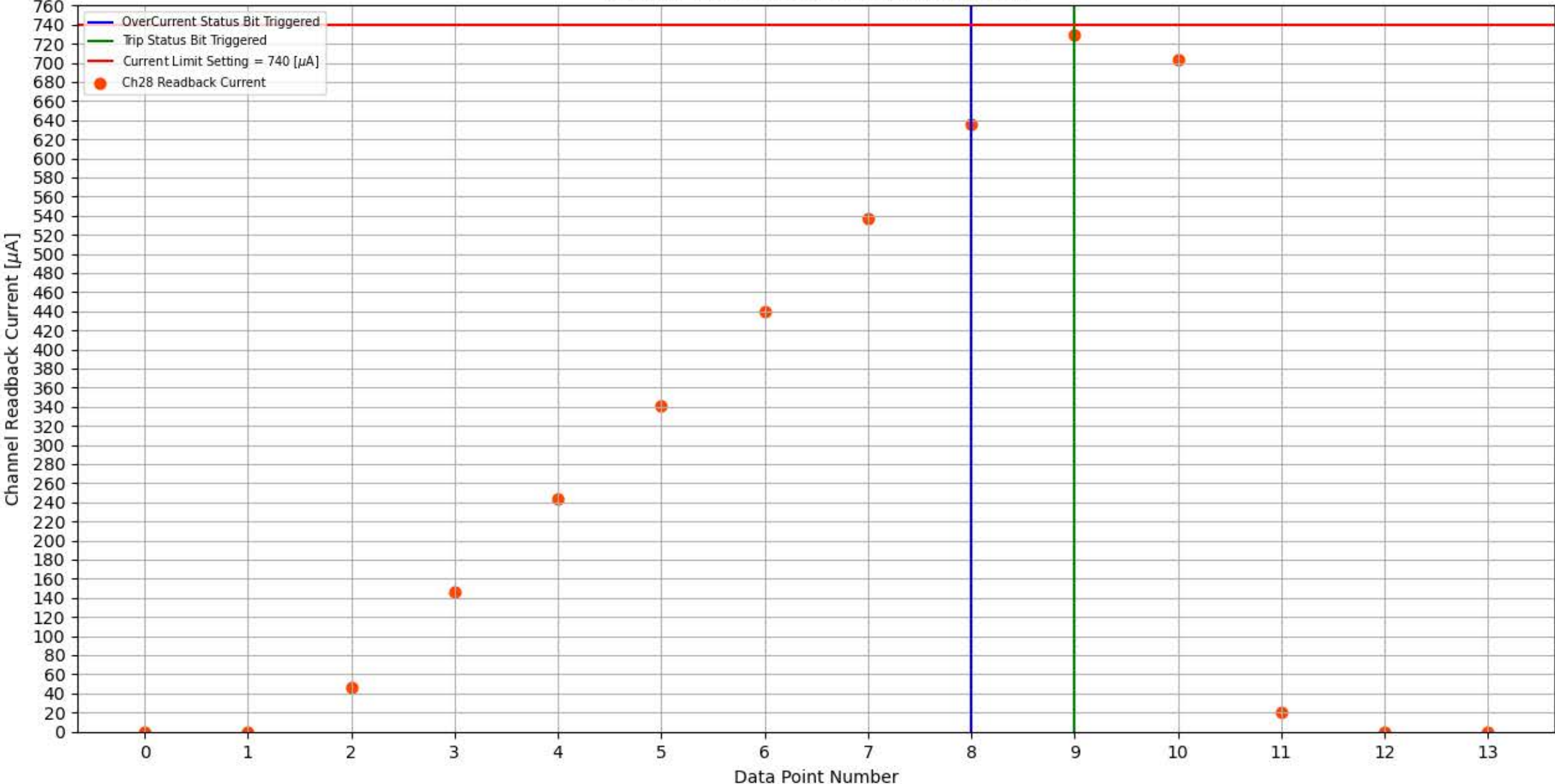
Module 184, Slot 2, Channel 28 Trip Test
