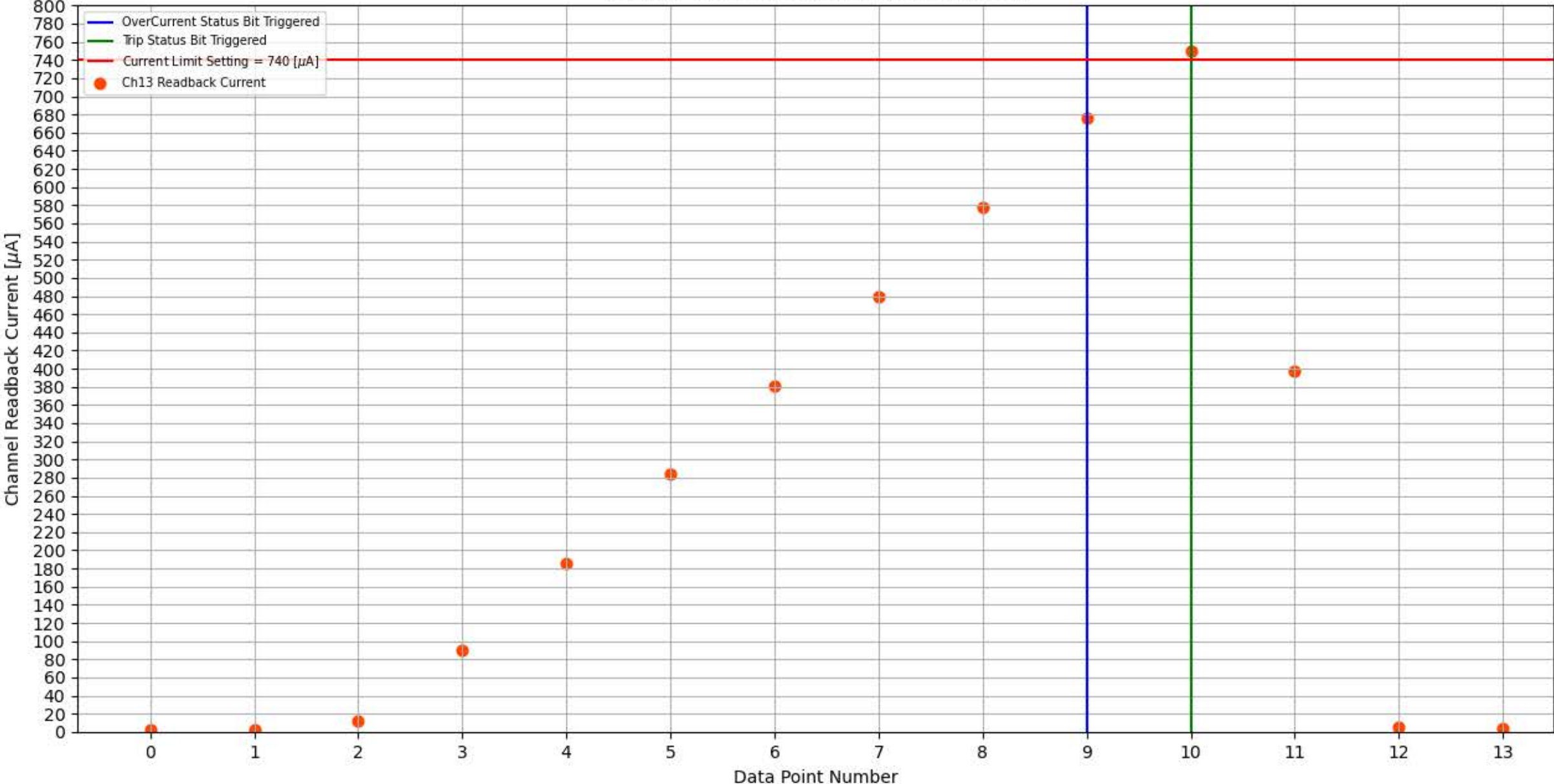
Module 184, Slot 2, Channel 13 Trip Test
