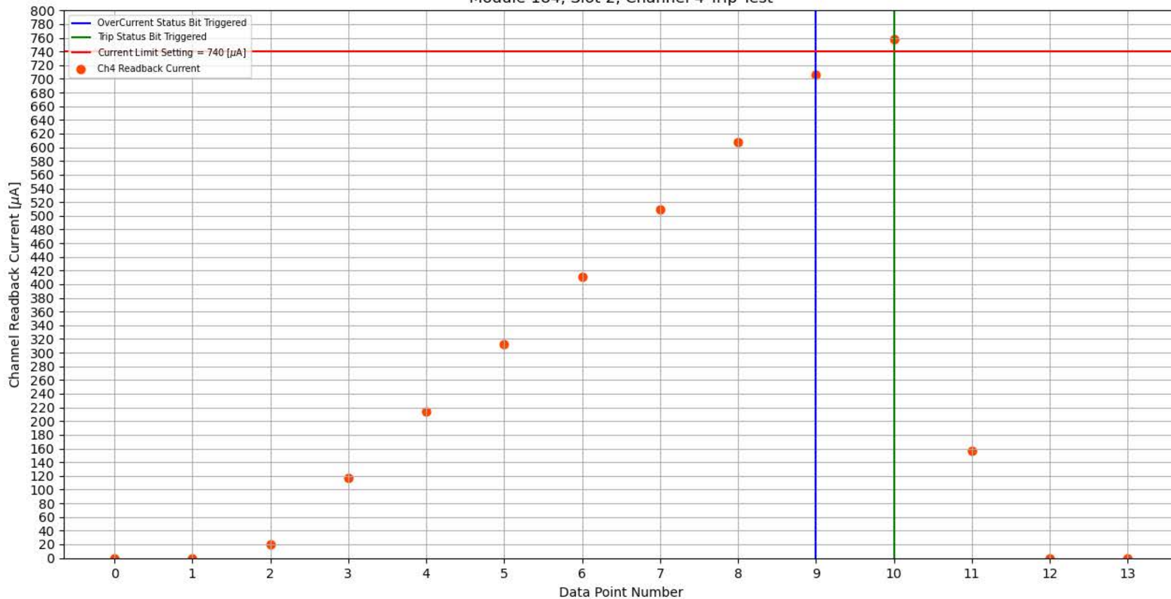
Module 184, Slot 2, Channel 4 Trip Test
