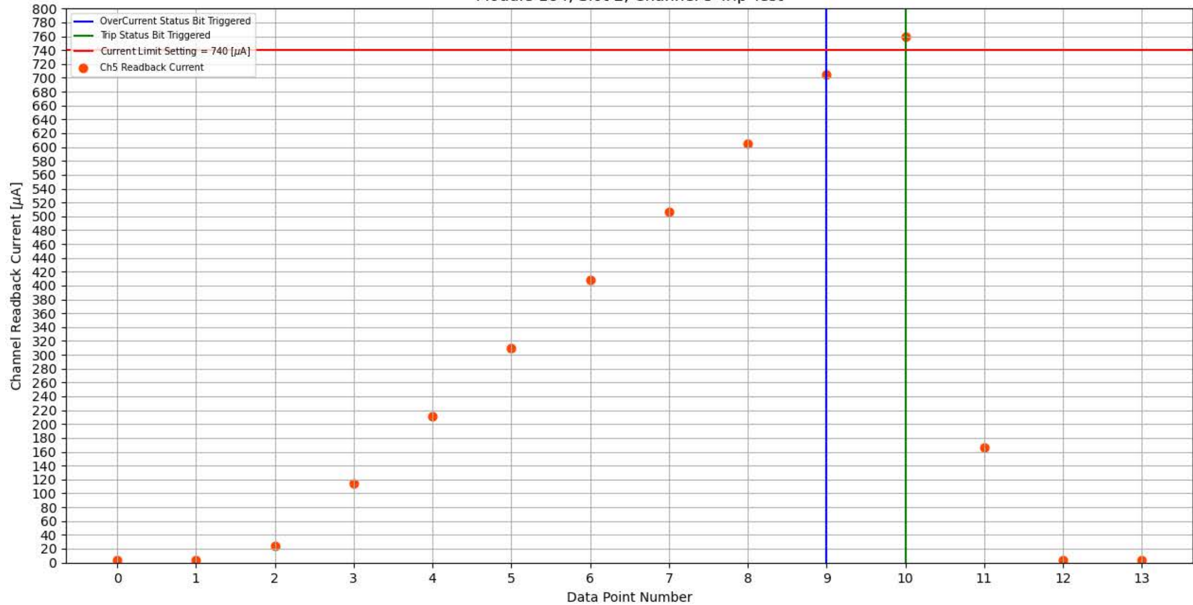
Module 184, Slot 2, Channel 5 Trip Test
