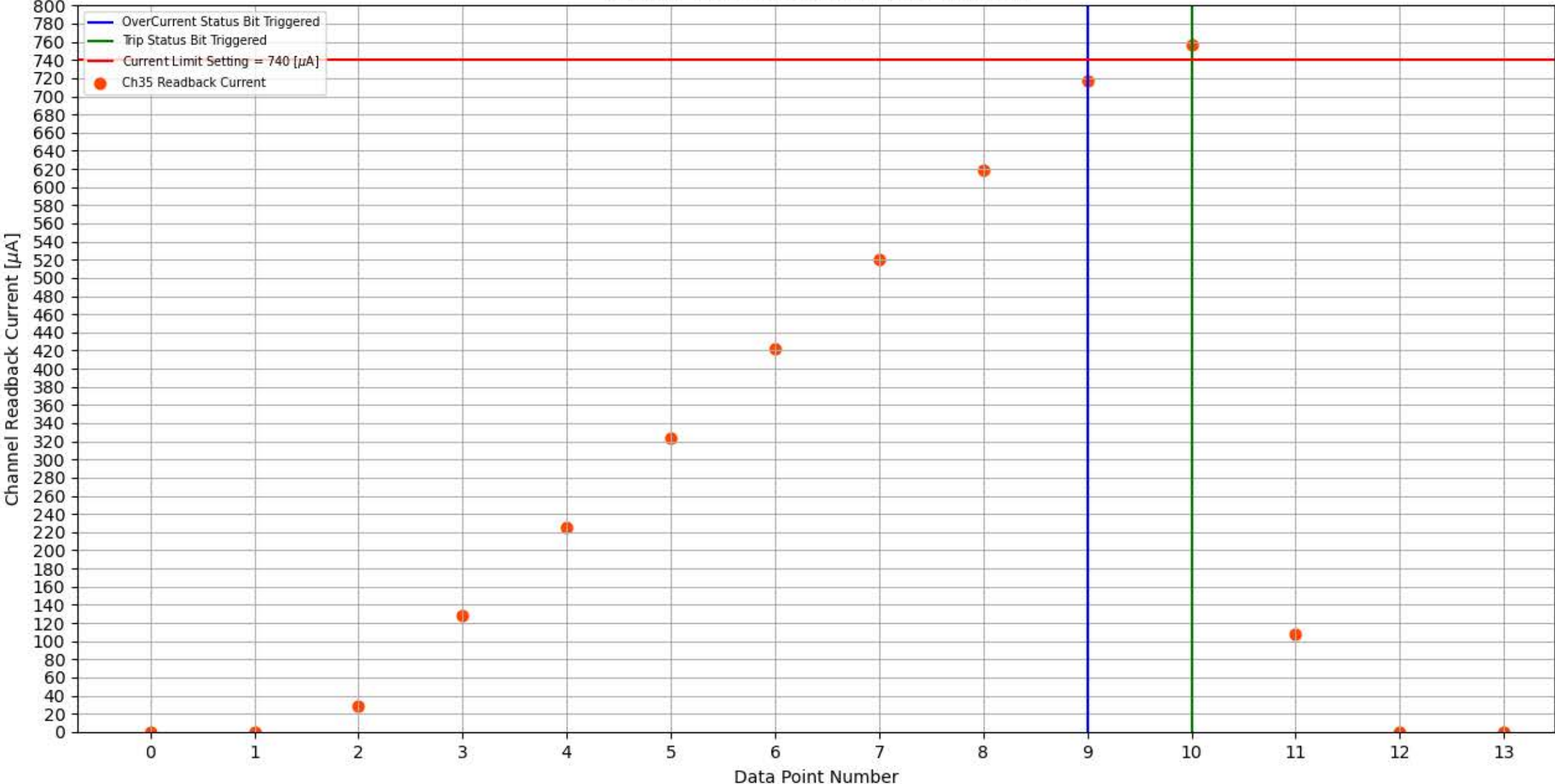
Module 184, Slot 2, Channel 35 Trip Test
