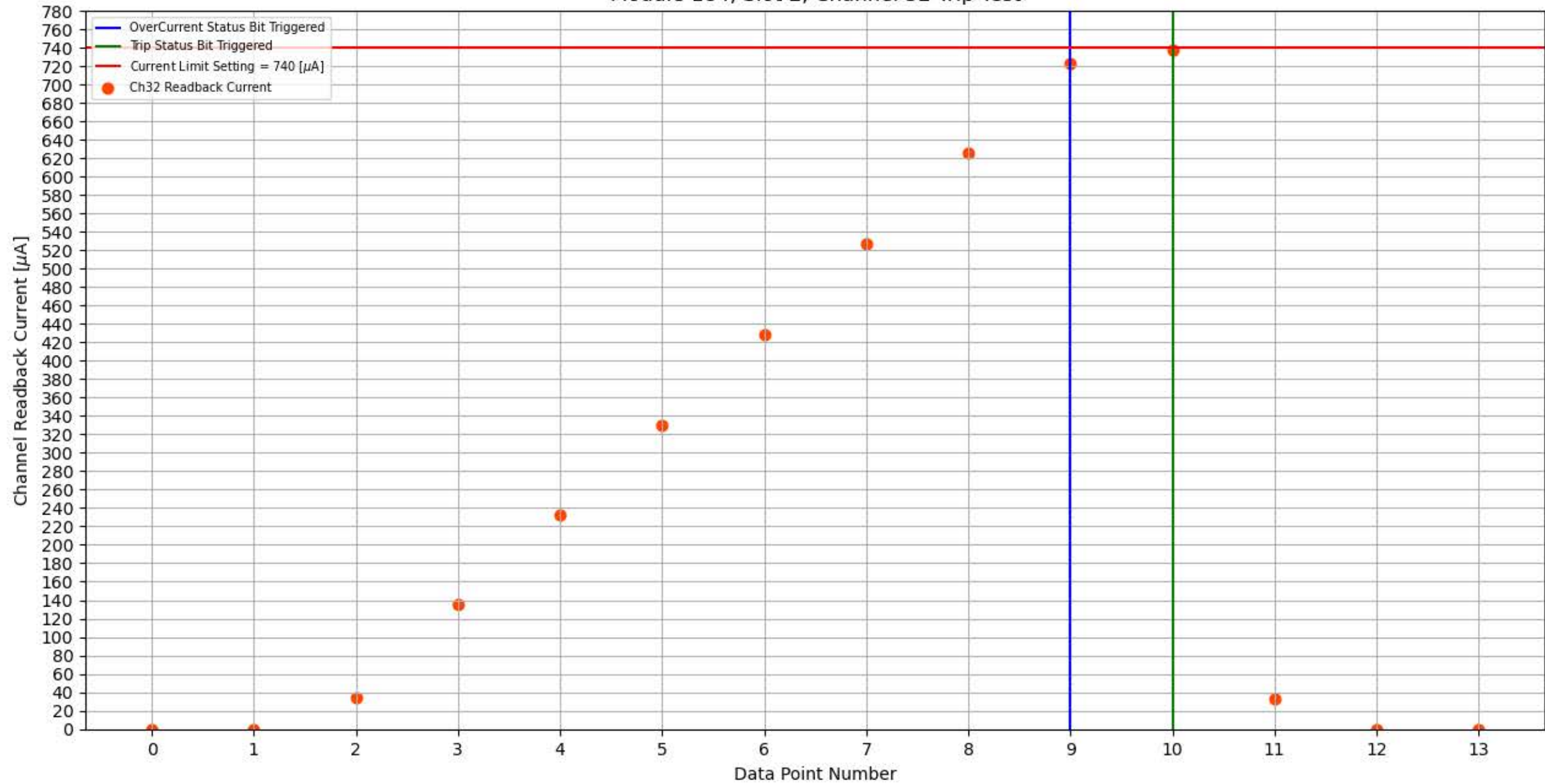
Module 184, Slot 2, Channel 32 Trip Test
