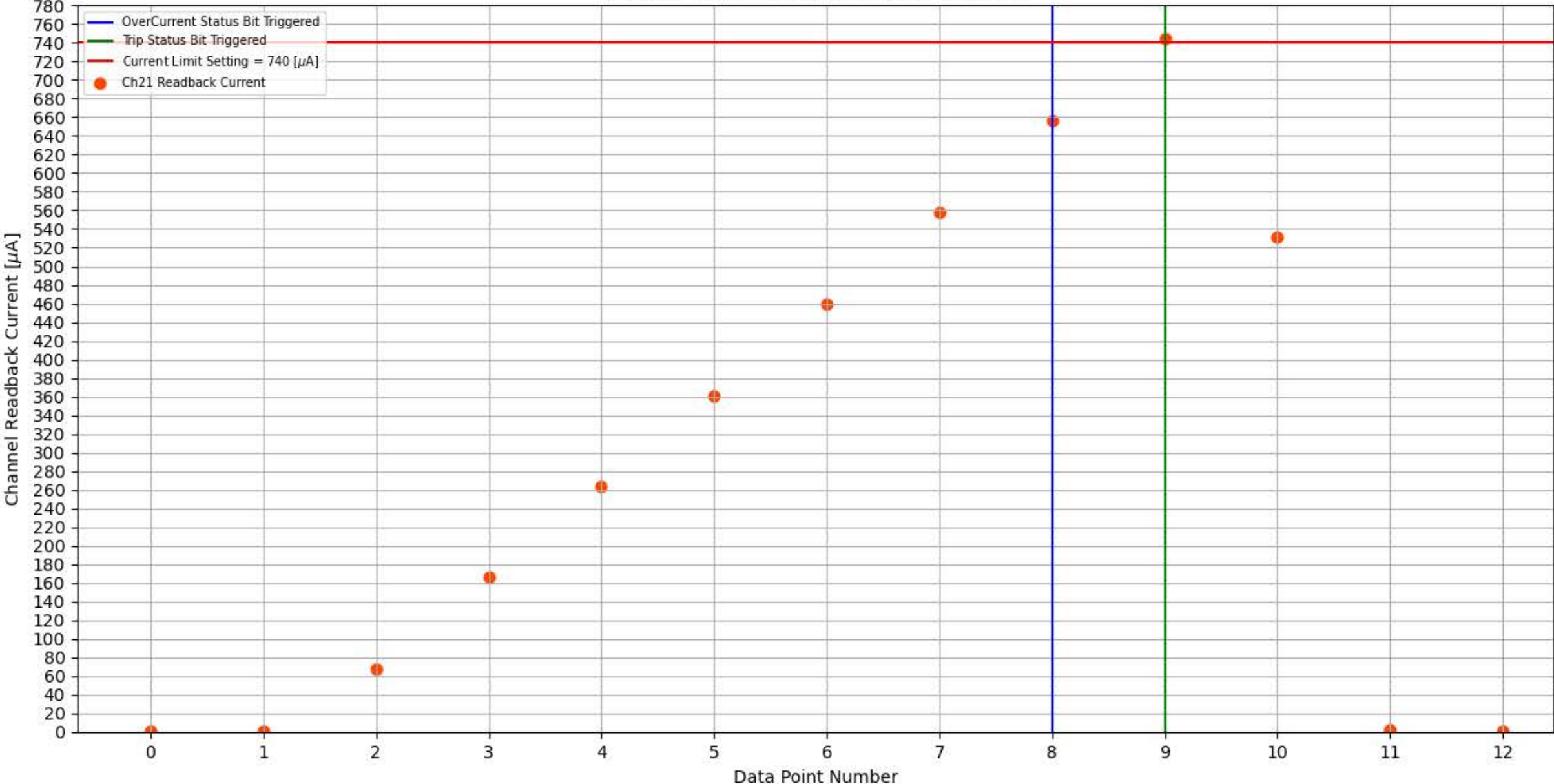
Module 184, Slot 2, Channel 21 Trip Test
