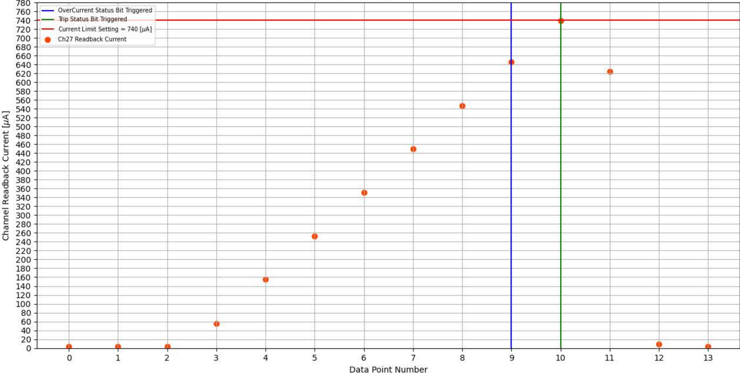
Module 184, Slot 2, Channel 27 Trip Test
